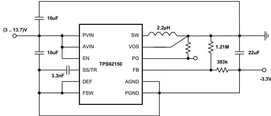
Figure 48. -3.3V Inverting Power Supply
